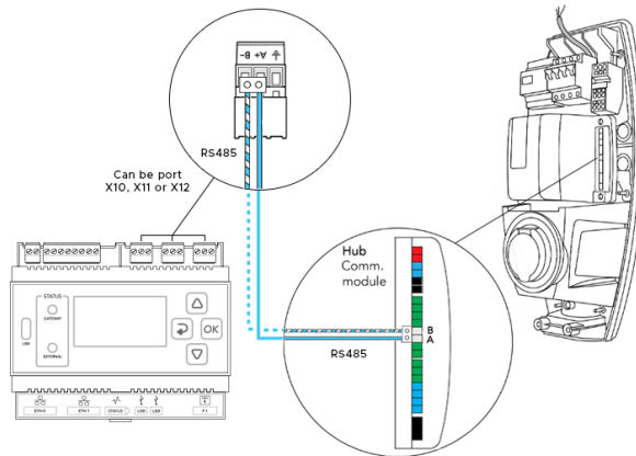
EVBox G4 RS485-connector
