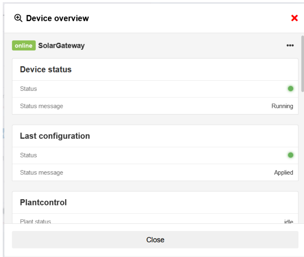
Device overview
