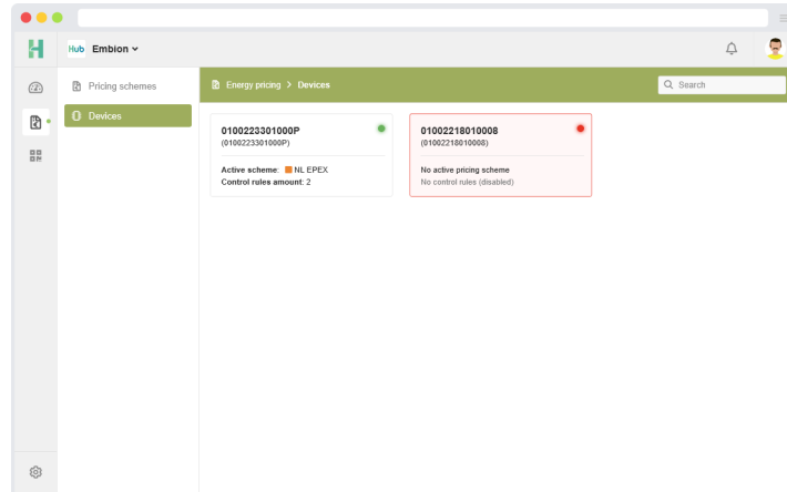
Devices
