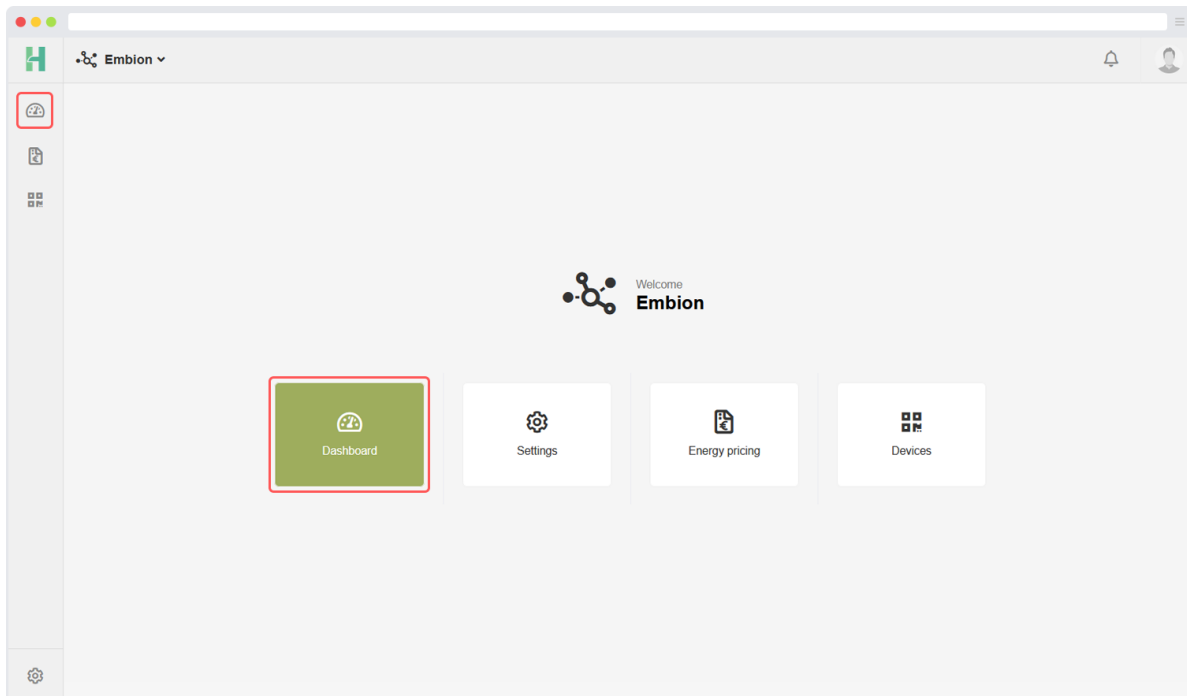
Dashboard application
