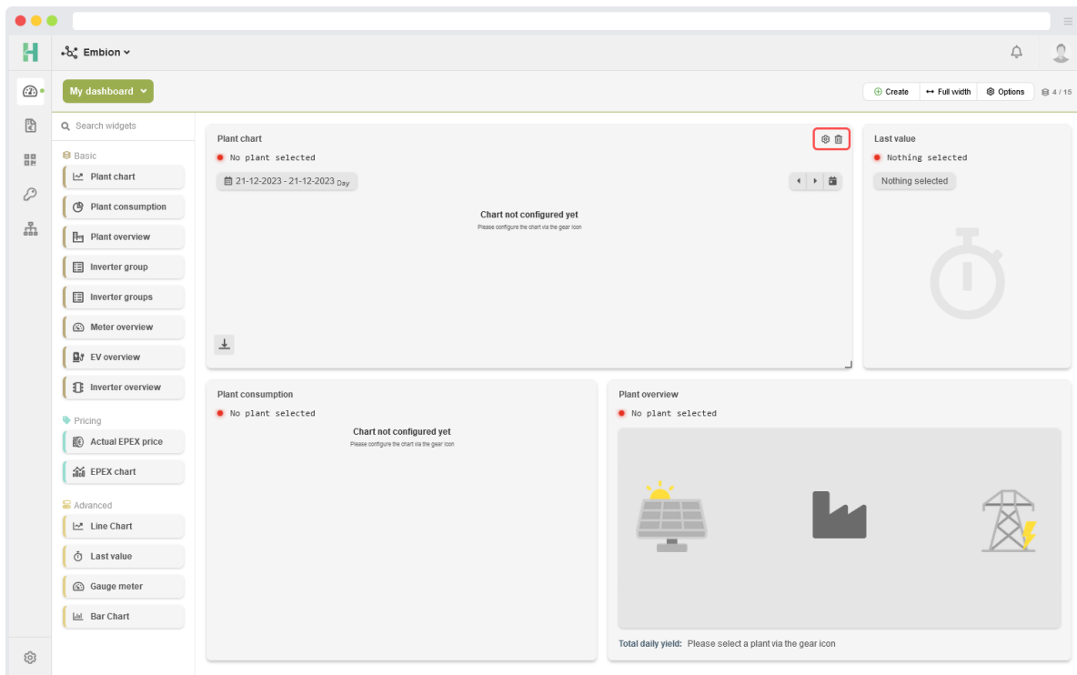
Figure 89: Configure widget
